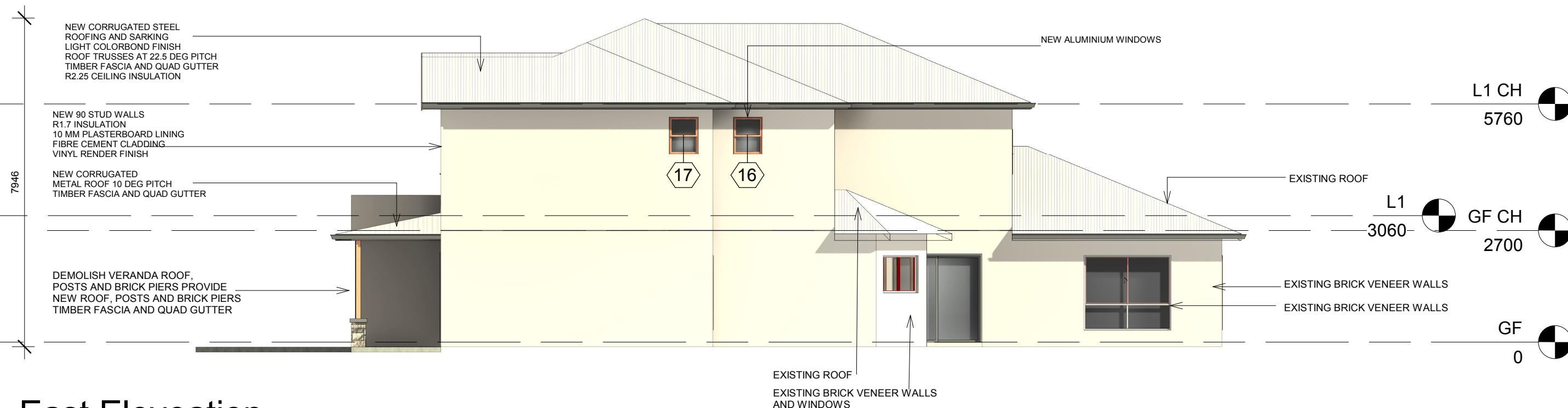
East Elevation
